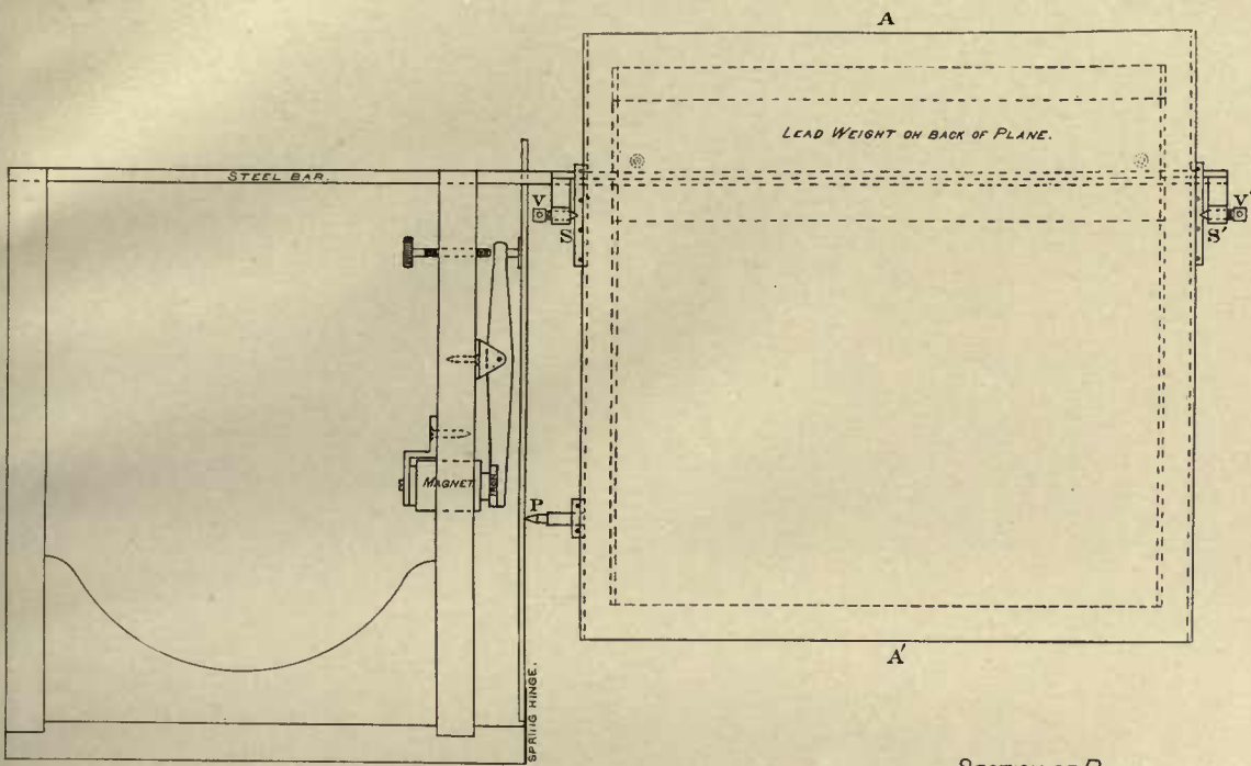
COUNTERPOISED ECCENTRIC PLANE.
